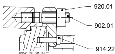
Fig. 20: Fastening elements for the clamped casing cover
