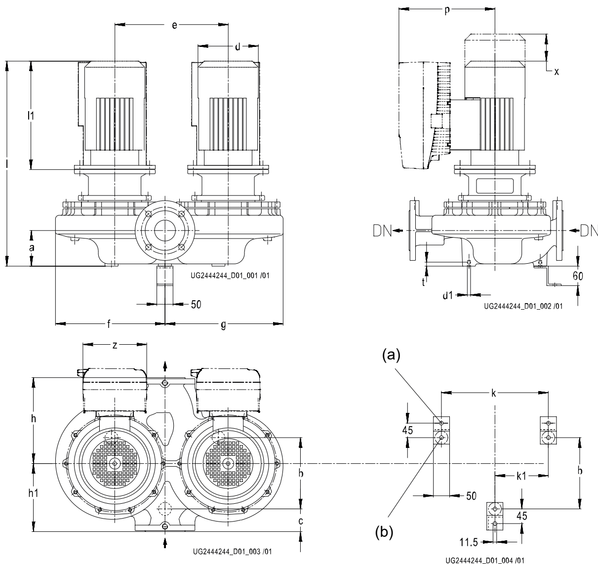
Fig. 6: Dimensions of pump set with PumpDrive 2 in [mm]
