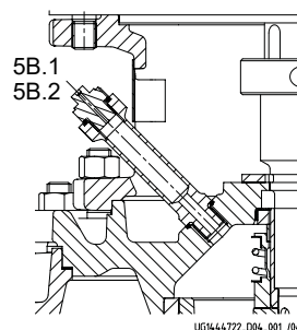
Fig. 16: Vent, mechanical seal chamber
