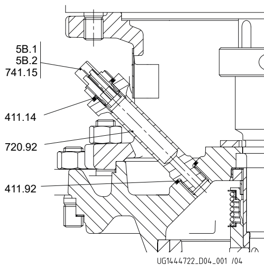
Fig. 19: Vent valve 5B.1 / 5B.2
