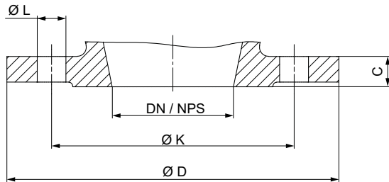
Fig. 9: Flange dimensions
