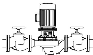
Fig. 13: Vertical installation / fastening without pump foot, sizes 032-032-160 to 080-080-250
