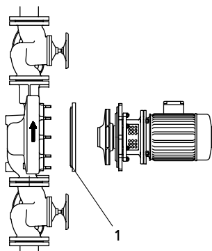
Fig. 12: Horizontal installation with blind flange, 1 = blind flange, accessory
