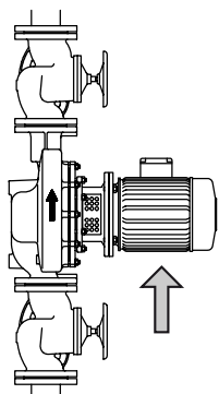
Fig. 10: Horizontal installation, direction of flow from bottom to top
