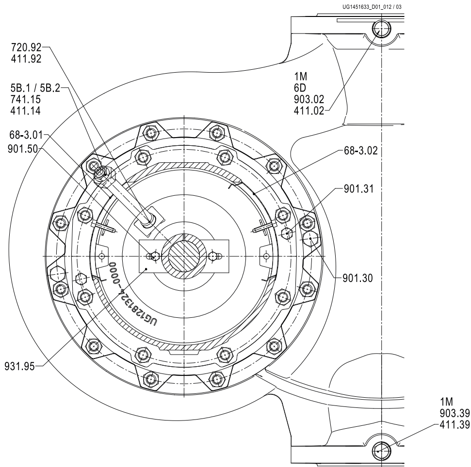
Fig. 18: General assembly drawing: side view (pump in operation)
