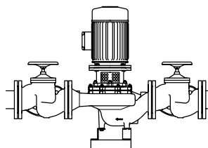
Fig. 14: Vertical installation / fastening with three angle feet (steel 37, accessories depend on the pump size), sizes 032-032-160 to 200-200-315
