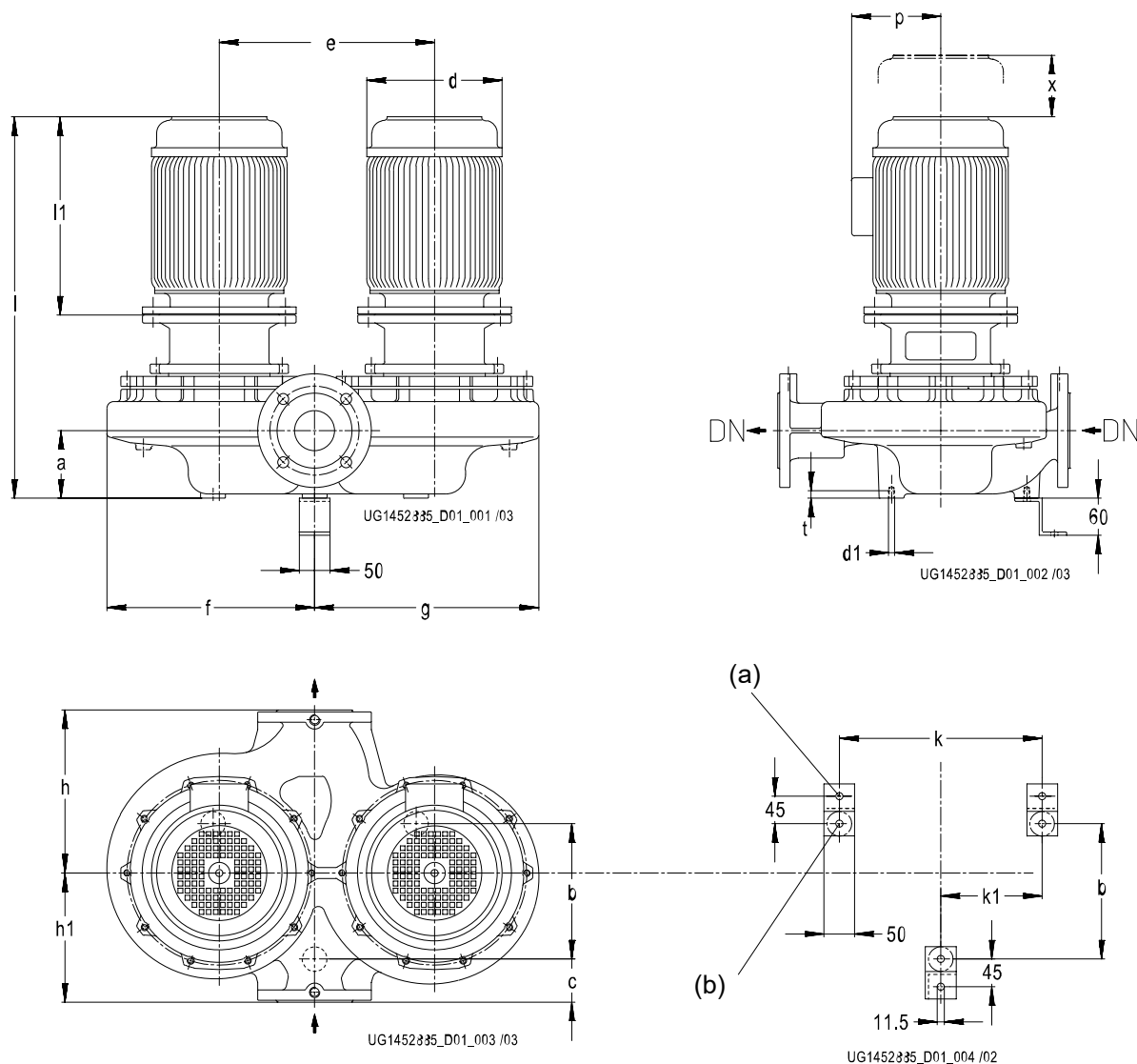
Fig. 2: Pump set dimensions in [mm]
