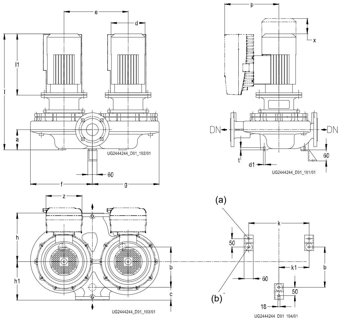
Fig. 7: Dimensions of pump set with PumpDrive 2 in [mm]
