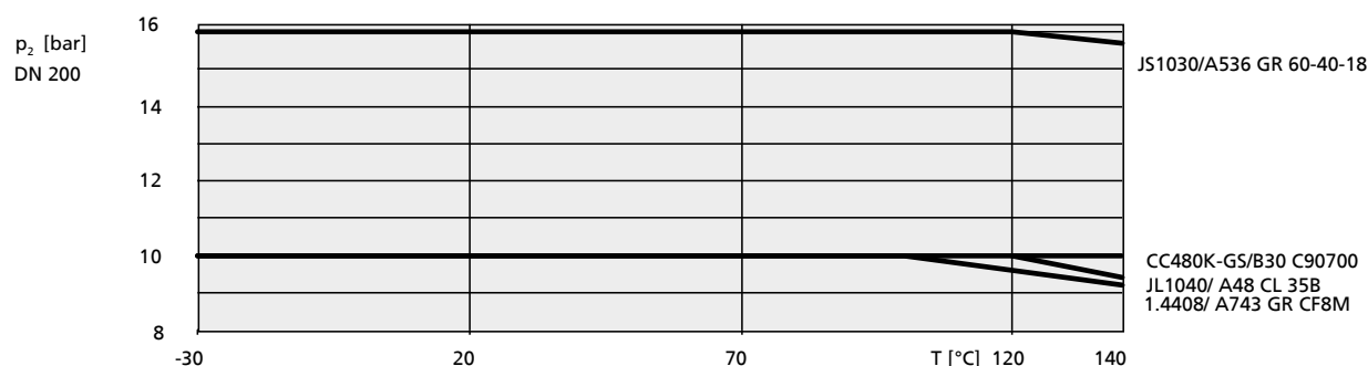
Fig. 2: Pump pressure limits and temperature limits DN 200 for ETN 35)
