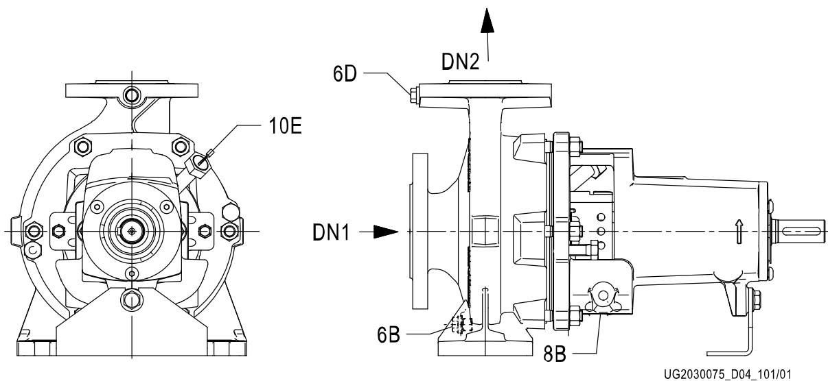
Fig. 8: Version with grease lubrication, no hole for connecting measuring equipment, no connection for pressure gauge
