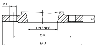
Fig. 12: Flange dimensions
