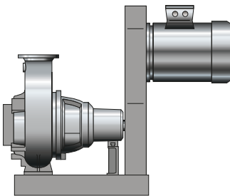
Fig. 2: Sewatec - 3H (3HZ): Pump set with baseplate, belt drive and belt guard
