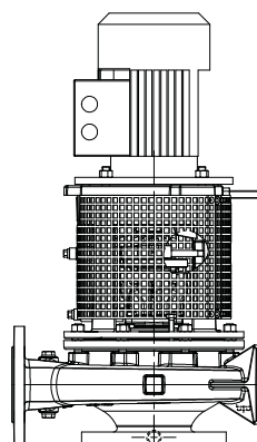
Fig. 7: Vertical installation, Etabloc SYT
