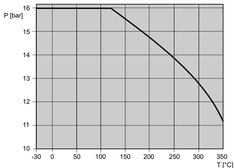
Fig. 1: Operating pressure limits and temperature limits
