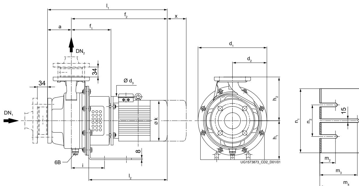
Fig. 6: Etachrom B with pump foot, dimensions [mm]
