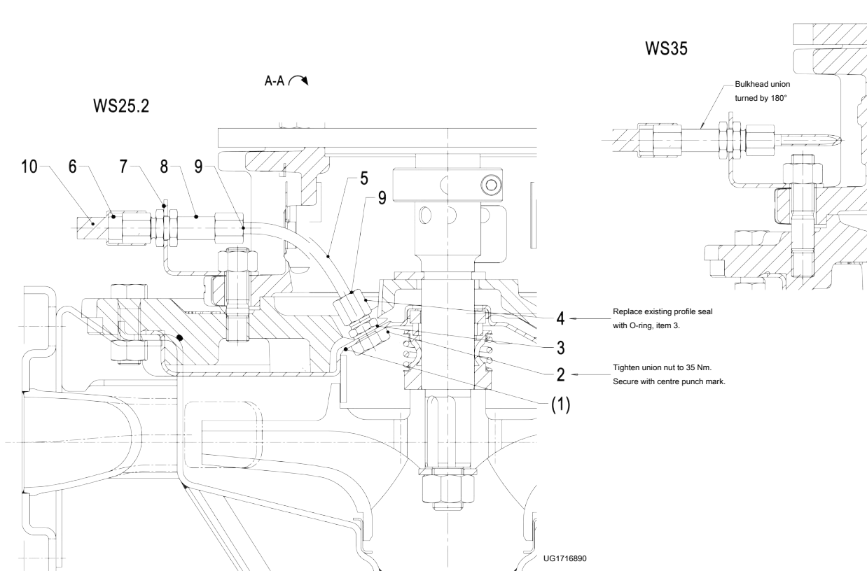
Fig. 28: Venting
