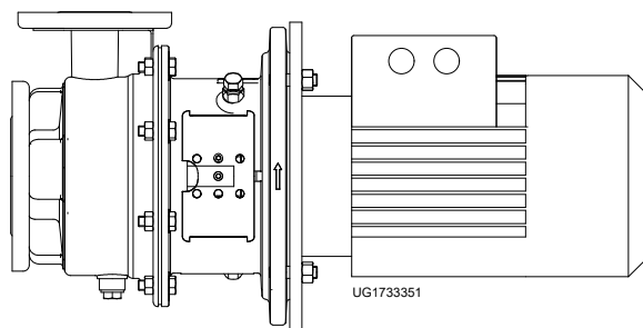
Fig. 23: Bottle rinsing variant, motor sizes 80 = 0.55 kW to 132 = 7.5 kW
