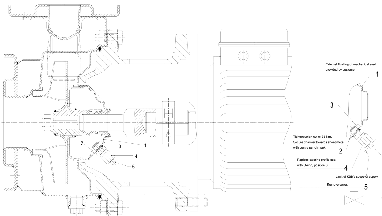
Fig. 30: External flushing
