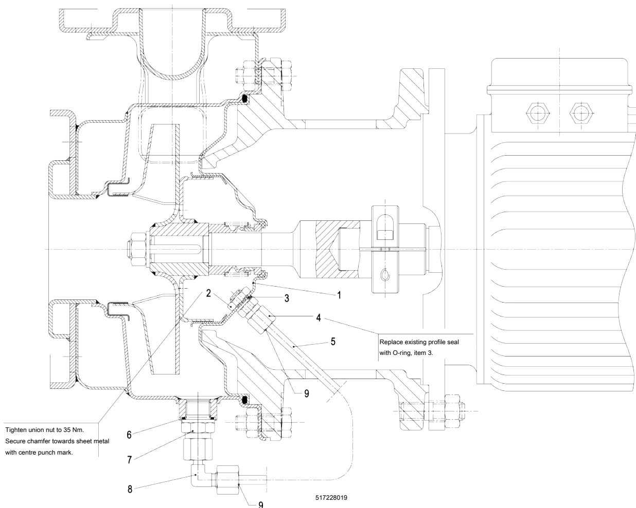
Fig. 29: External circulation
