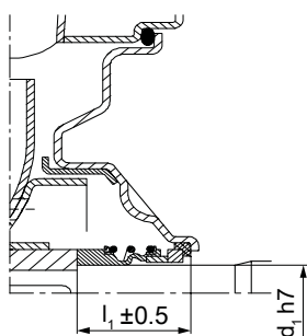
Fig. 2: Mechanical seal dimensions [mm]
