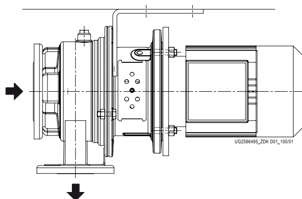
Fig. 19: Pump foot, fastened above, up to motor size 112 = 4 kW The terminal box must be turned by 90° or 270°.
